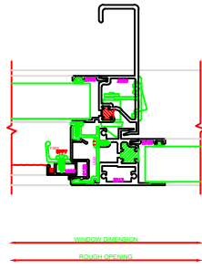
606 MEETING RAIL SERIES 5500
